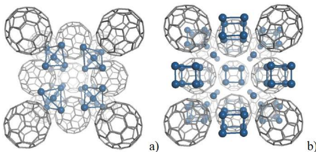
FIGURE 8.2: Left: The low temperature phase of \text{Li}_{12}\text{C}_{60} [203]. Right: A graphical representation of the high temperature phase as suggested by \mu\text{SR} and INS experiments [204]. The frontal \text{C}_{60} has been omitted for clarity.
