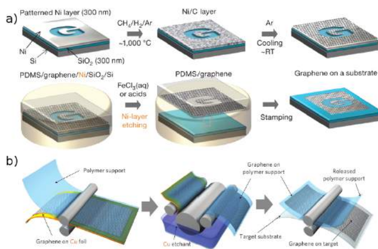
FIGURE 1.10: (a) Scheme of preparation of graphene by CVD and transfer via polymer support. The carbon solves into the Ni during the CVD and forms graphene on the surface after cooling. With a polymer support the graphene can be stamped onto another substrate, after etching of the Ni layer. An appropriate patterning of the Ni foil allows a control of the shape of the graphene. (b) Roll-to-roll process of graphene films grown on copper foils and transferred on a target substrate. Taken from http://www.physik.fu-berlin.de .
