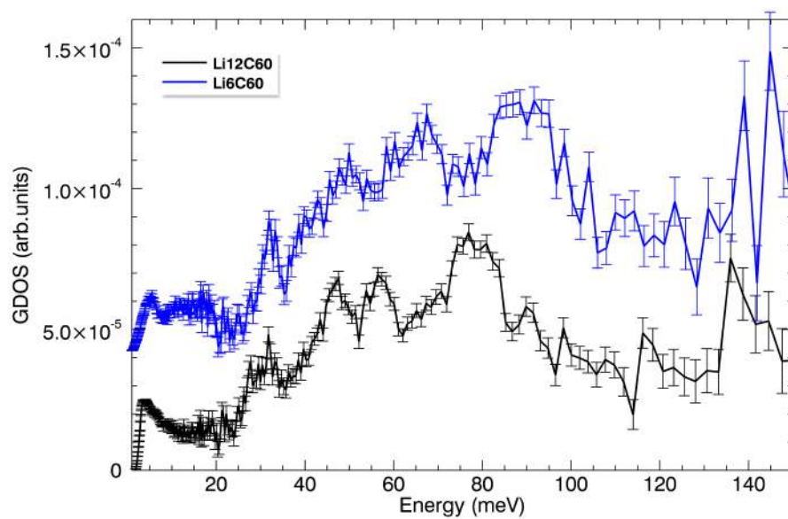
FIGURE 8.6: GDOS of \text{Li}_6\text{C}_{60} and \text{Li}_{12}\text{C}_{60} measured on IN4C at 320 K and using an incident \lambda = 2.41 \text{ \AA} . The GDOS of \text{Li}_6\text{C}_{60} displays important similarities with respect to \text{Li}_{12}\text{C}_{60} , in particular in the Li-modes region [10-50 meV]. The clear modification of the intramolecular modes [ E \geq 40 \text{ meV} ] with respect to \text{Li}_{12}\text{C}_{60} suggests a probable lower symmetry and the distortion of the buckyball.
