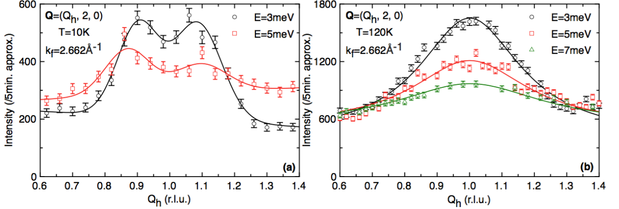
Figure 5.9: (a) Raw data depicting spin-wave scattering at different constant energy transfers along the (h00) high symmetry direction of the orthorhombic system at T=10 K (AF1 phase). Lines represent fits with Gaussian functions. (b) PM scattering at different constant energy transfers along the (h00) high symmetry direction of the orthorhombic system at T=120 K. Lines represent fits with Lorentzian functions. Data were obtained at 2T1.
