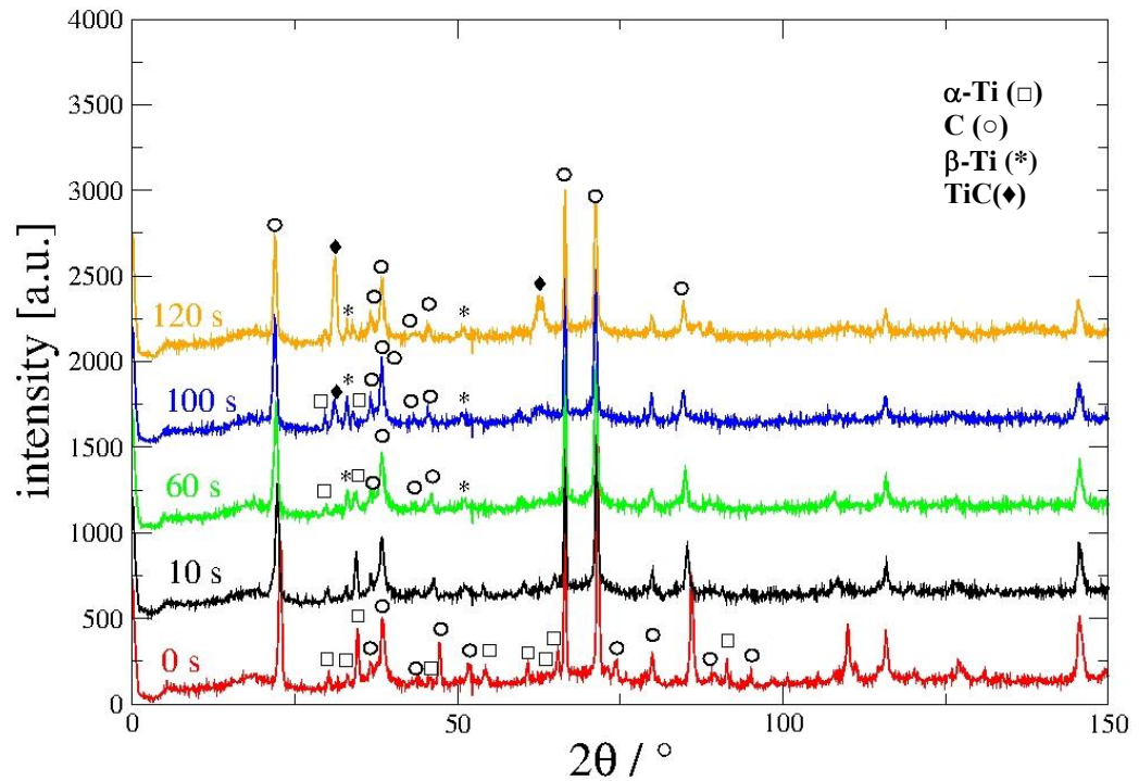
Figure 4.5 Sample 3 . For clarity, the diffractograms have been normalized at 0, 10, 60, 100, and 120 s by shifting their intensity and adding a constant of, respectively, 0, 500, 1000, 1500, 2000.
