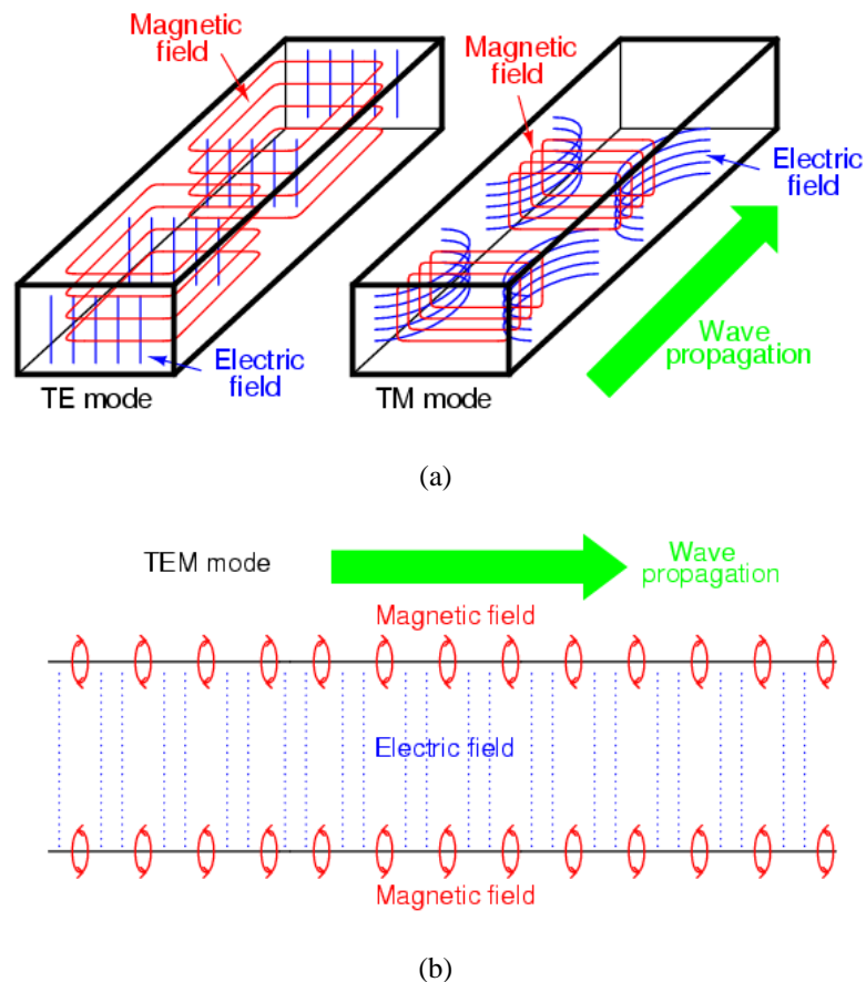
Figure 2.10 a) TE (transverse electric - left) and TM (transverse magnetic - right) mode. (Picture from: http://www.allaboutcircuits.com/vol_2/chpt_14/8.html ); b) TEM mode waveguide: both field planes (electrical and magnetic) are perpendicular (transverse) to the direction of signal propagation.
