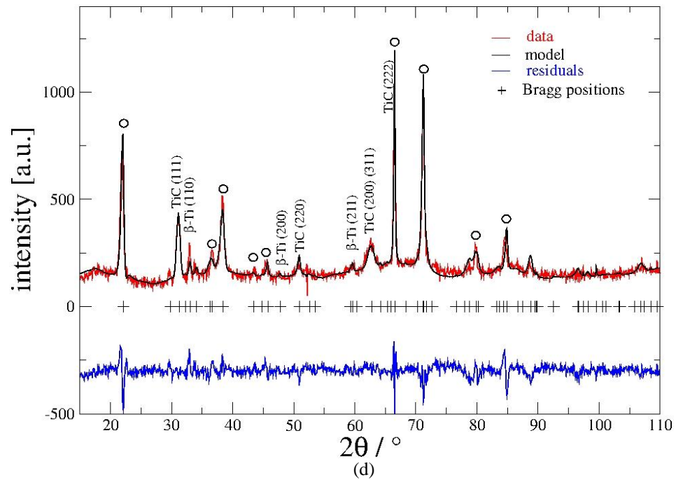
Figure 4.10 (a) Profile plots for Rietveld refinement against neutron data for sample 3 , (a) at t = 0 ; (b) at t = 60 s; (c) at t = 100 s; (d) at t = 120 s. Reflections from C ( \circ ) are indicated.
