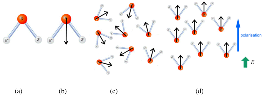
Figure 2.2 (a) H 2 O molecules showing a permanent dipole. (b) Permanent dipoles are usually represented by an arrow. (c) In thermal equilibrium, dipoles are randomly arranged. The dipole moments from different molecules cancel out and the net polarization is zero. (d) When applying an external electric field, dipoles rotate in order to align with the field E and with each other: the net polarization is therefore non-zero. (Picture adapted from: http://www.doitpoms.ac.uk/tlplib/dielectrics/polarisation_mechanisms.php ).
