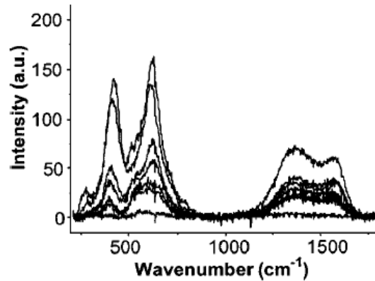
Figure 2.29 Raman spectra of commercially available TiC (as in ref:[35]).
