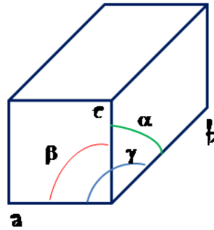
Figure 2.18 a , b , and c and the angles between them ( \alpha , between axes b and c ; \beta , between axes a and c and \gamma , between axes a and b ) describe the unit cell.
