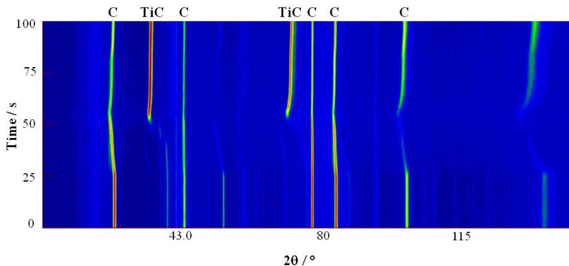
Figure 4.6. Full reaction diffraction profile for sample 4 . The formation of TiC (~ 50 s) is indicated by new peaks appearing at ca. 36 ° and 72 ° 2 \theta .
