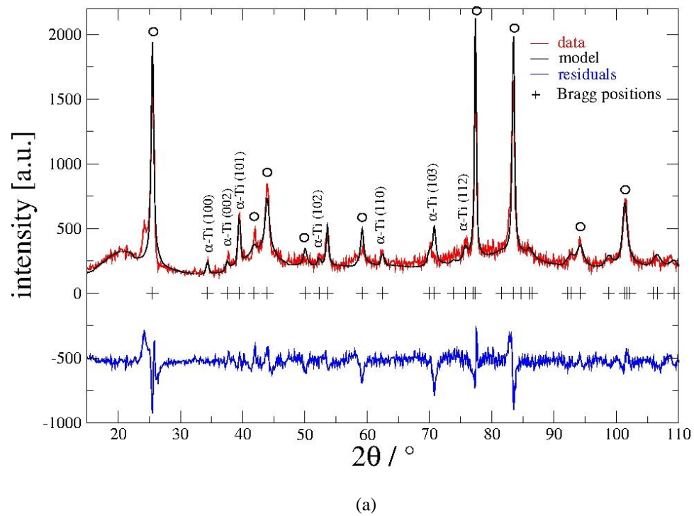
Figure 4.10 (a) Profile plots for Rietveld refinement against neutron data for sample 3 , (a) at t = 0 ; (b) at t = 60 s; (c) at t = 100 s; (d) at t = 120 s. Reflections from C ( \circ ) are indicated.
