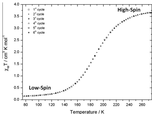
Figure 3. Temperature dependent magnetic behavior of a [Fe(PM-AzA) 2 (NCS) 2 ] single crystal showing the gradual spin-crossover. A thermal cycling has been applied leading to six magnetic curves.
