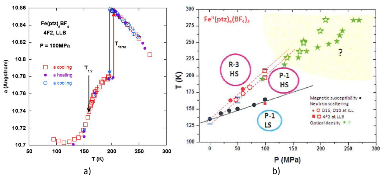
Figure 34 [\text{Fe}(\text{ptz})_6](\text{BF}_4)_2 :
